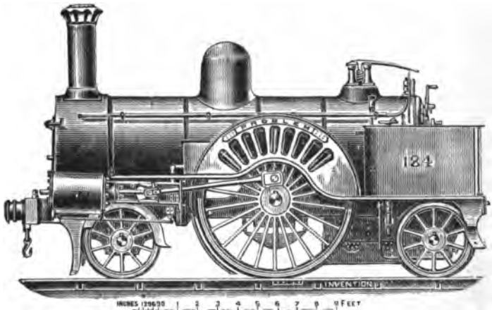
Fig. 61.—“ Problem,” London and North-Western Railway, Northern Division, November, 1869.
